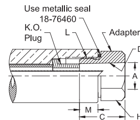
EJECTOR TYPE ADAPTERS 7/8-14 THREAD
